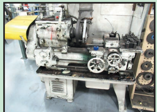
LEBLOND 13" X 20" CUSTOM CHAMFER LATHE
