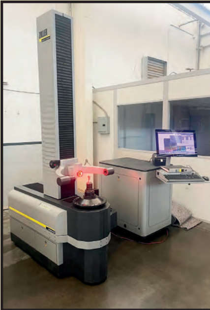
ZOLLER VENTURON MDL. 800/16 CNC TOOL PRESETTER
