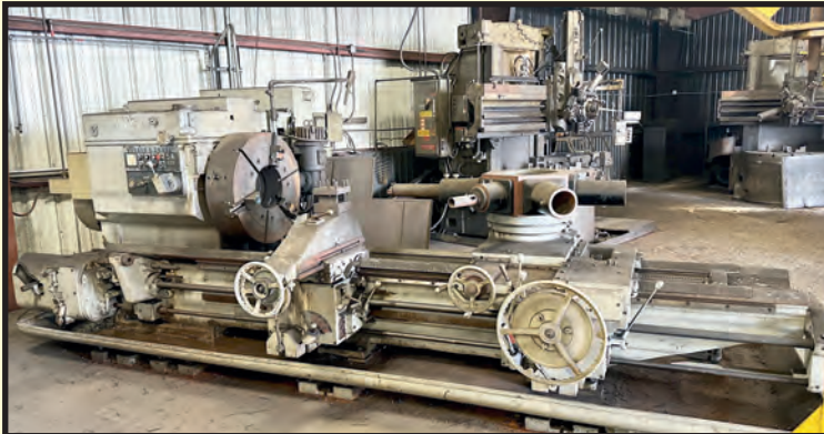
WARNER & SWASEY MDL. 5A TURRET LATHE
