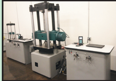
TINIUS OLSON 400K AND 60K SUPER L TENSILE TESTERS
