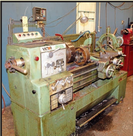
VICTOR 16" X 40" ENGINE LATHE
