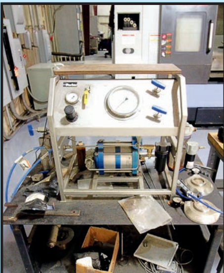
PARKER AIR PRESSURE TEST STAND
